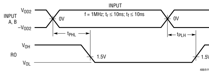
Figure 3. Receiver Propagation Delays
